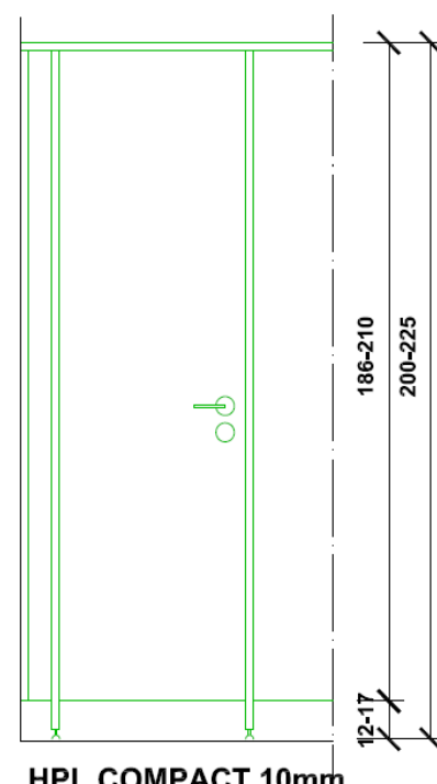
HPL COMPACT 10mm HPL COMPACT 13mm
