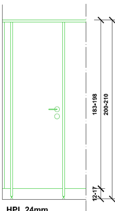
HPL 24mm HPL PLW 24mm
